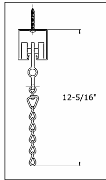
Cross Section of 280 Ceiling Mount
