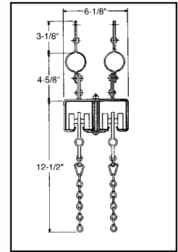
Cross Section of 280 Track at Center Overlap Pipe Mounted
